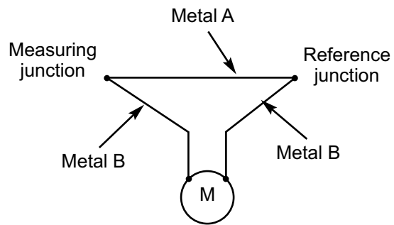
Thermocouple schematic
