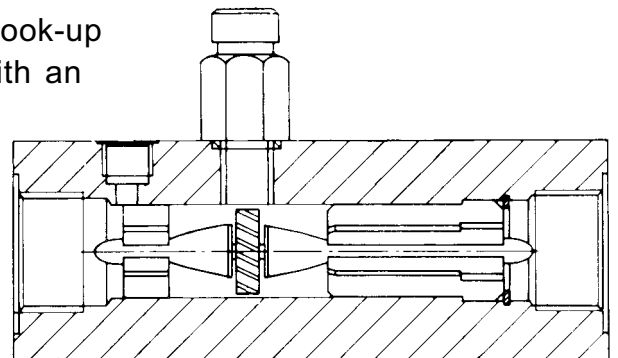
Webster LT400 schematic
