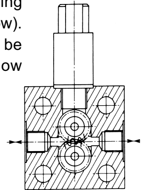
Webster LT10 schematic
